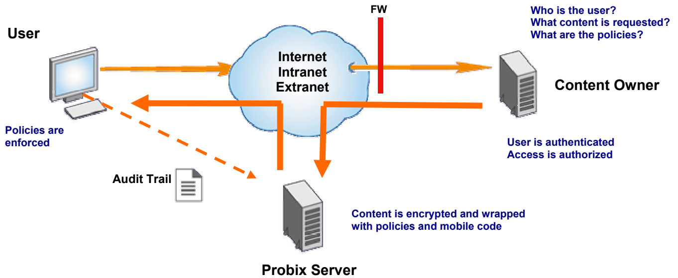
Diagram 1: Probix Trustee™ Information Flow
